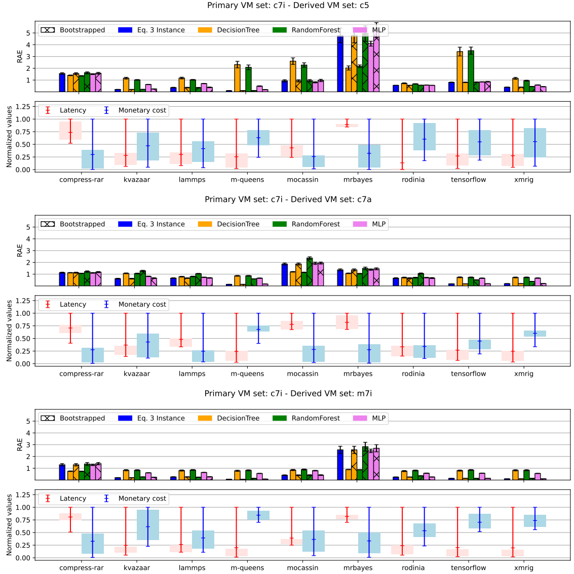
Fig. 7. Results for C5, C7a and M7i families for all benchmark applications, using C7i family as a primary VM set, three samples ( k = 3 ) for the primary VM set and one sample for each.
